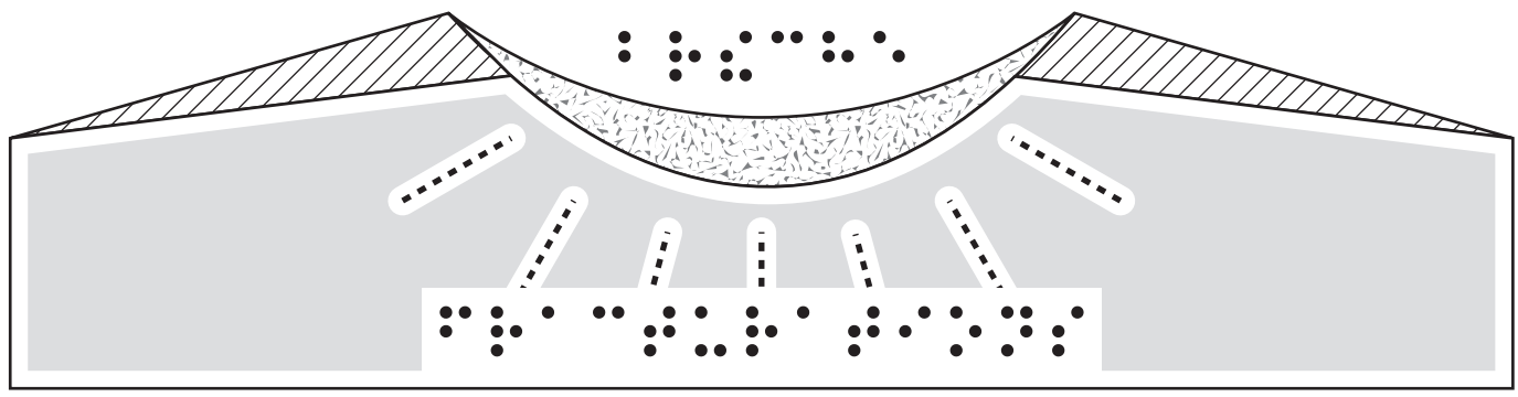
fracturations
