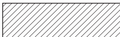
arid regions
